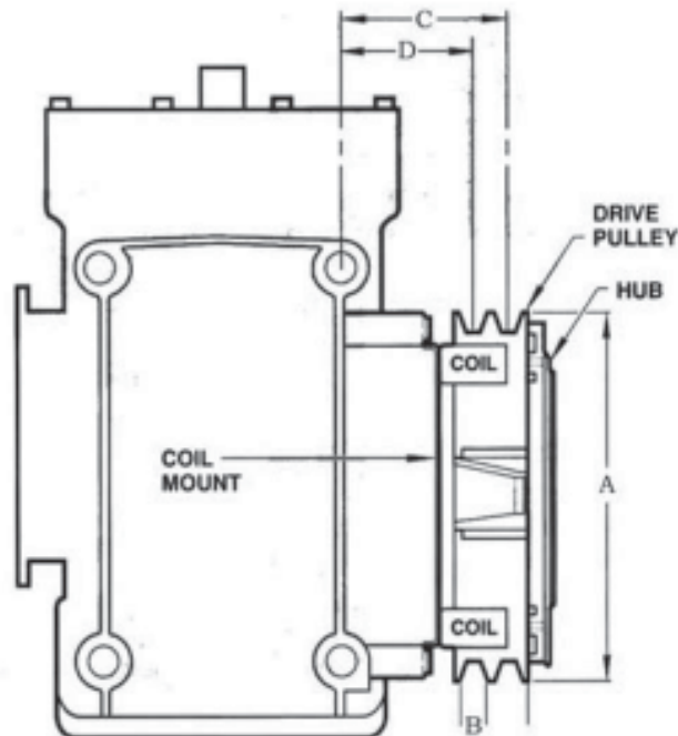
CLUTCH REFERENCE DIMENSIONS (IN INCHES)
